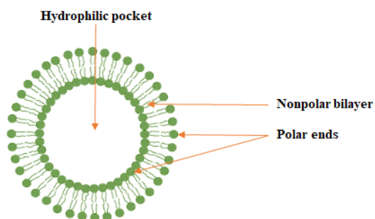
Figure 1. Liposome.
